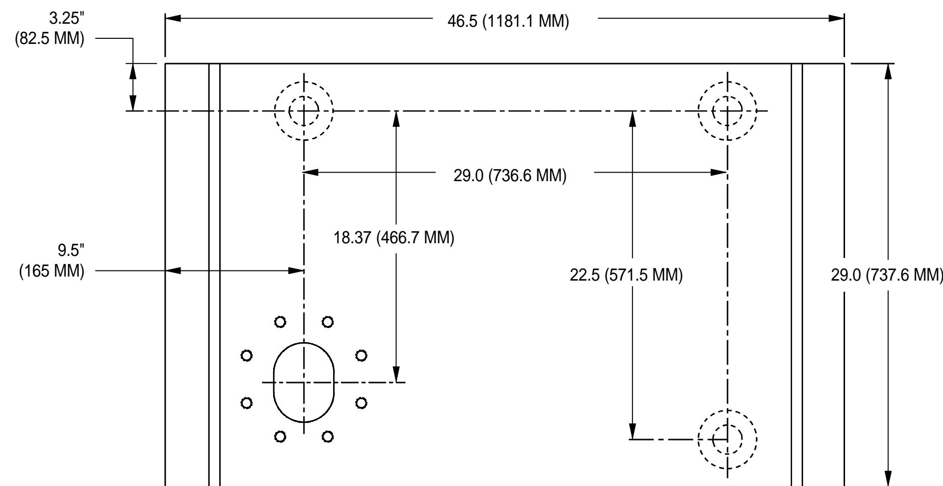
MOUNTING FOOTPRINT - TOP VIEW WITH COVER REMOVED
