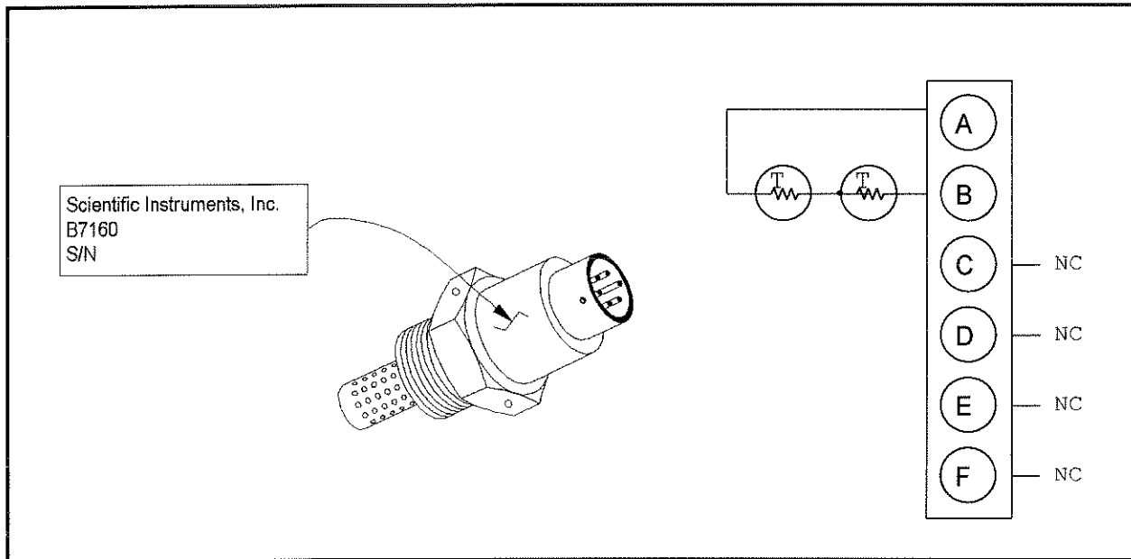
Outline and Schematic Drawing Figure 1
