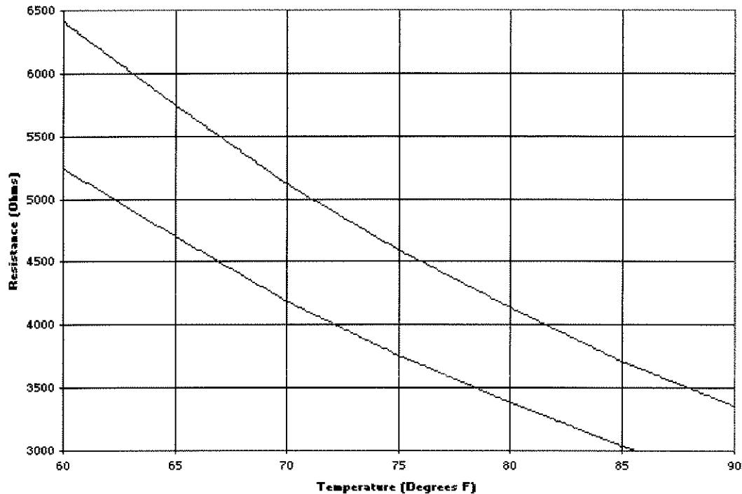
Resistance vs Temperature Figure 3
