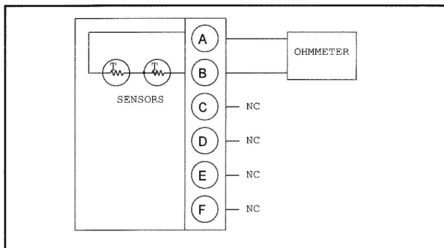
Schematic for Electrical Test
